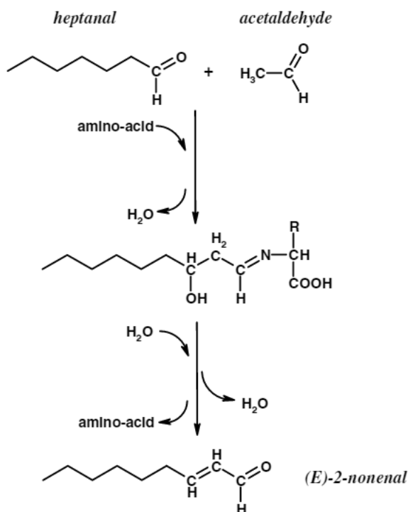
Fig. 5. Formation of (E) -2-nonenal in beer by aldol condensation of acetaldehyde and heptanal according to Hashimoto and Kuroiwa (1975).
